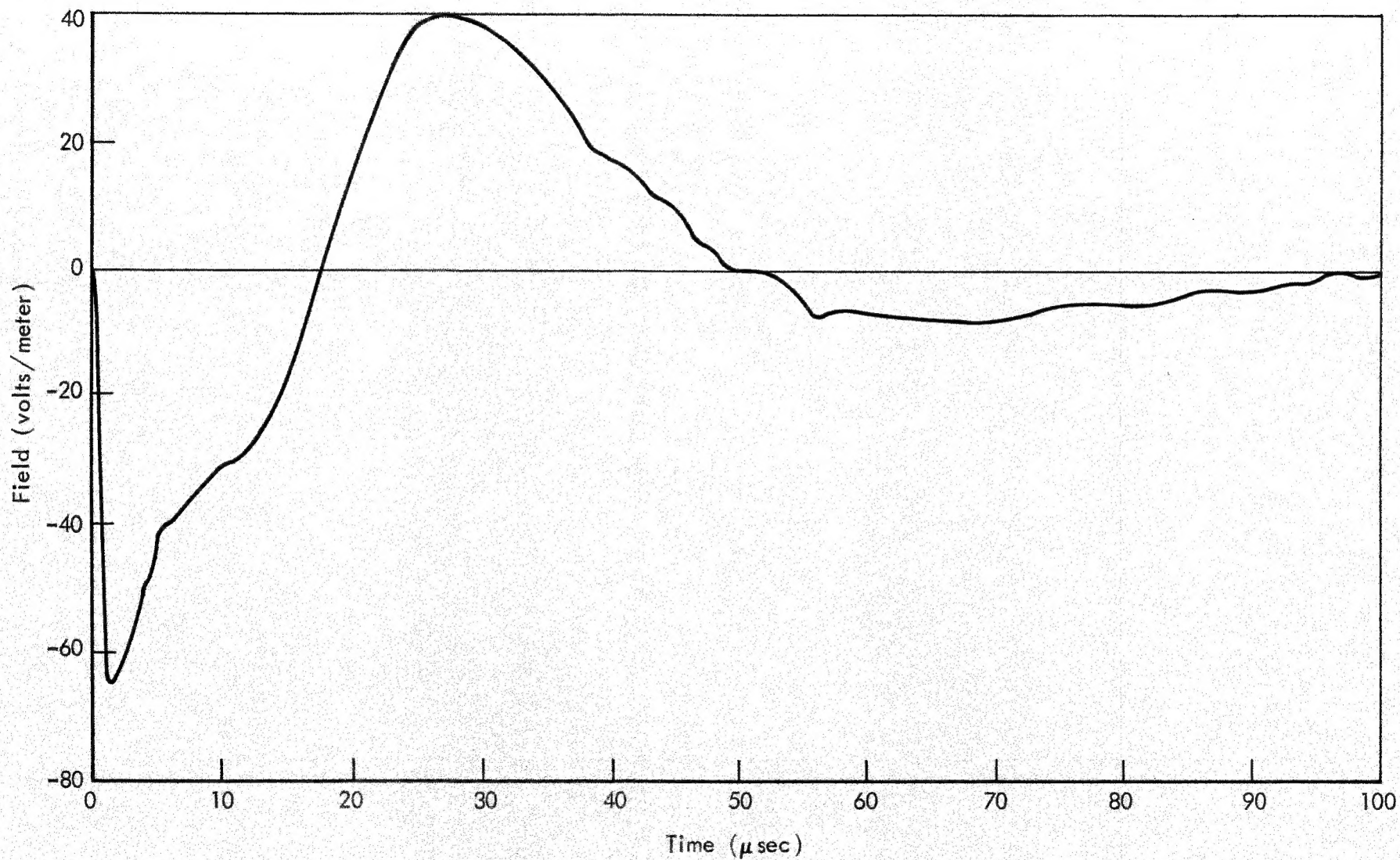
Fig. 7—Observed pulse at 44.6 km (From Ref.5)
